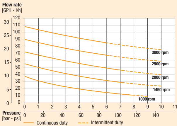
GA0072 - 24 V 42x100 mm BRUSHLESS MOTOR (90-93-02)
